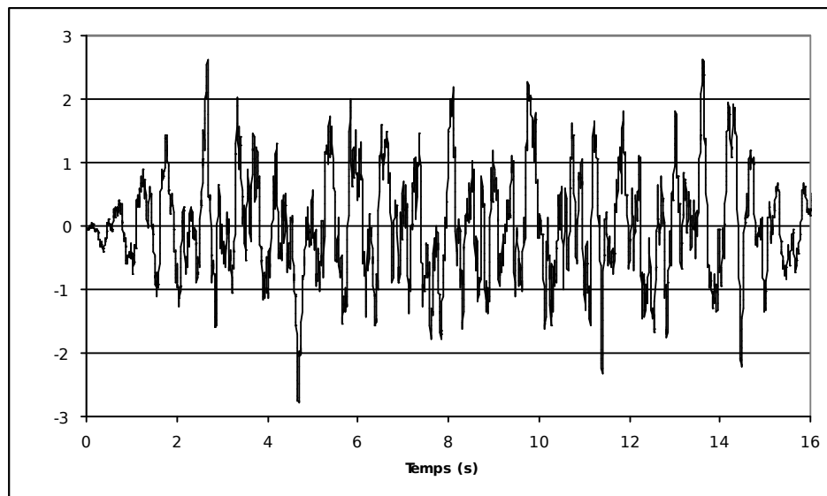
Figure 1.3-a : hasccélérogramme ac_s2_c_1 imposed on the structure
