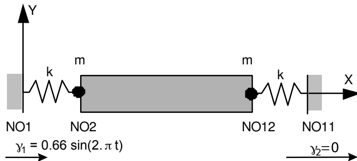
Figure 3.1-a: Modeling of the seismic anti device
