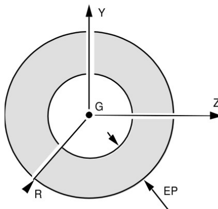
Figure 9.4.5-1 : Section CIRCLE.
