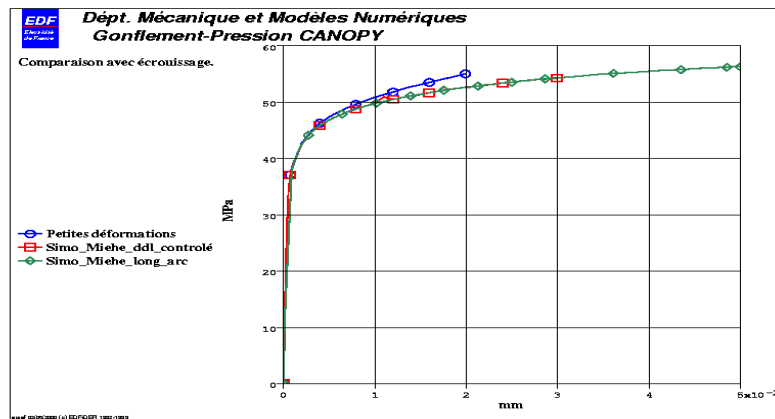
Figure 4.6-c. Elastoplastic incremental calculation in great transformations (Simo-Miehe) with two types of piloting, compared with a calculation in small transformations.
