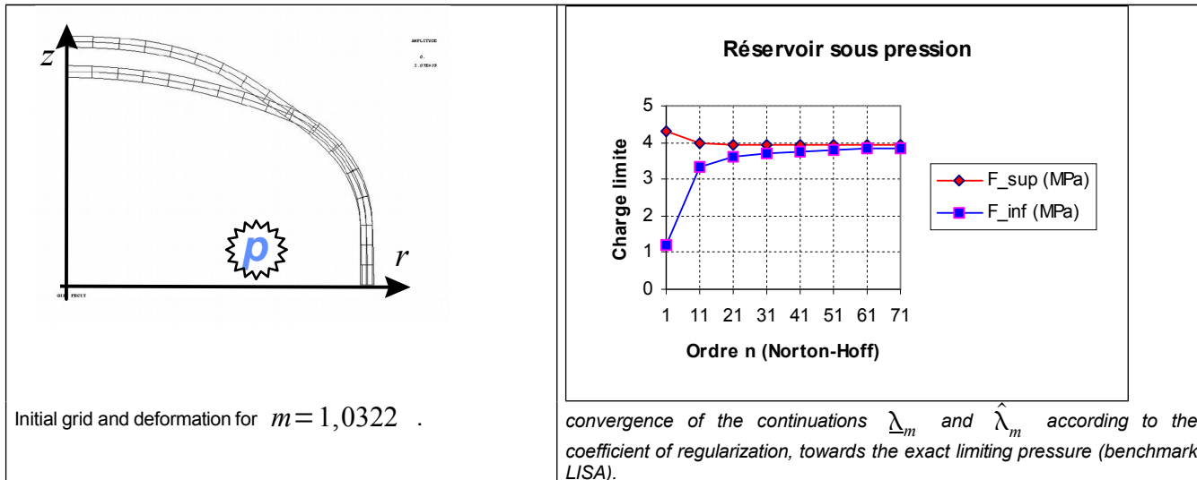
Figure 4.1-a : results of EDF calculation carried out within the framework of the benchmark LISA with the old method
