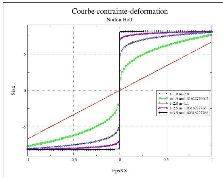
Figure 3.6-a. Stress-strain curve for various values of the moment t
