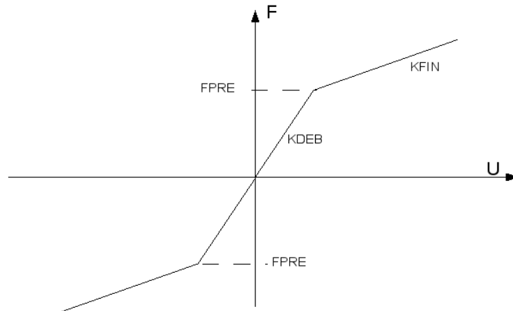
Figure 3.1-a : Bilinear elastic behavior
