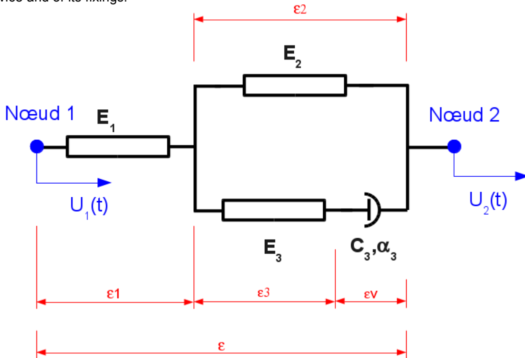
Figure 5.1-a : Discrete nonlinear viscoelastic model rheological.
