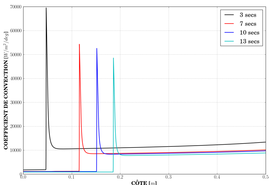
Figure 4.3-1: Convection coefficients at several moments of a calculation with condensation of the vapor.
