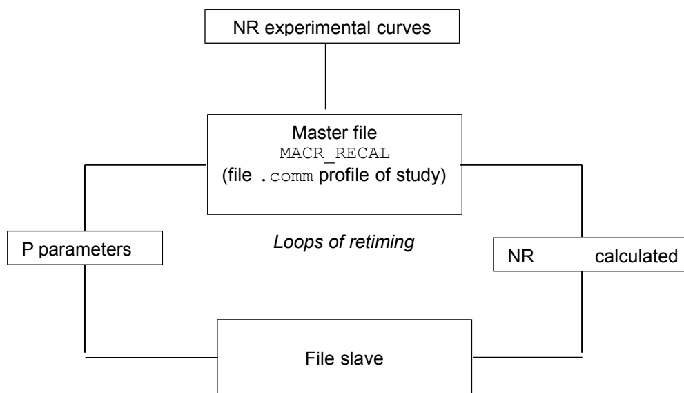
Figure 3.2-a. Diagram of operation of the procedure of retiming for the classical case
