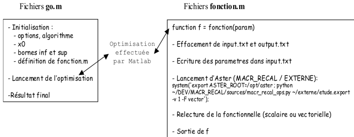
Figure 7.3-a: MACR_RECAL “Principle of the EXTERNAL mode” applied to Matlab©
