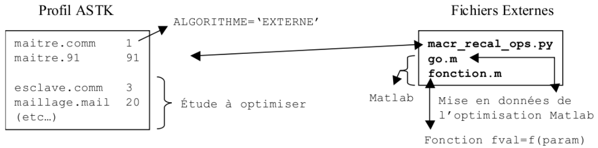
Figure 3.3-a : MACR_RECAL method EXTERNAL
