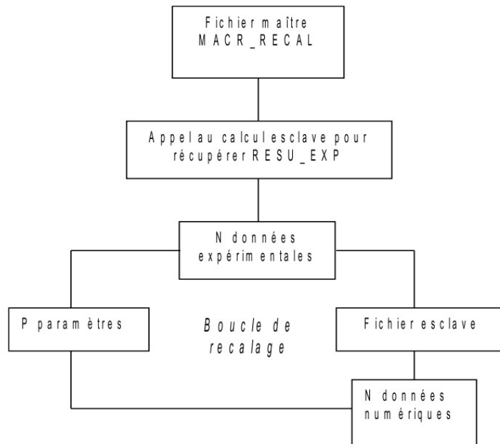
Figure 3.4-a. Diagram of operation of the procedure of retiming in dynamics
