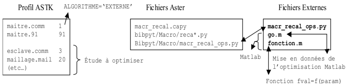
Figure 7.2.1-a: MACR_RECAL “External algorithm”
