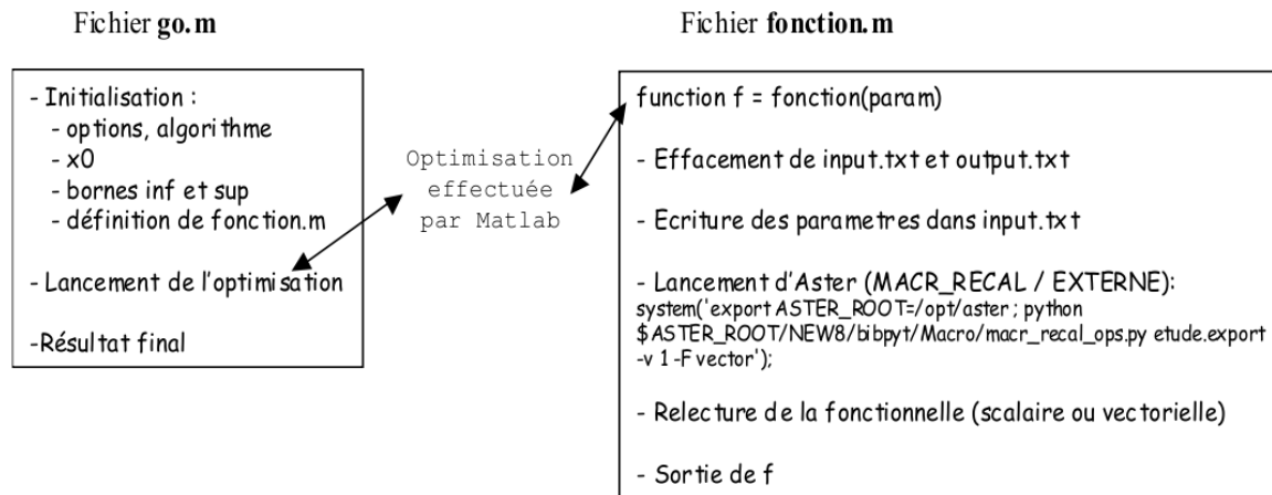
Figure 7.2.1-b: MACR_RECAL "Principle of the EXTERNAL mode", example Matlab
