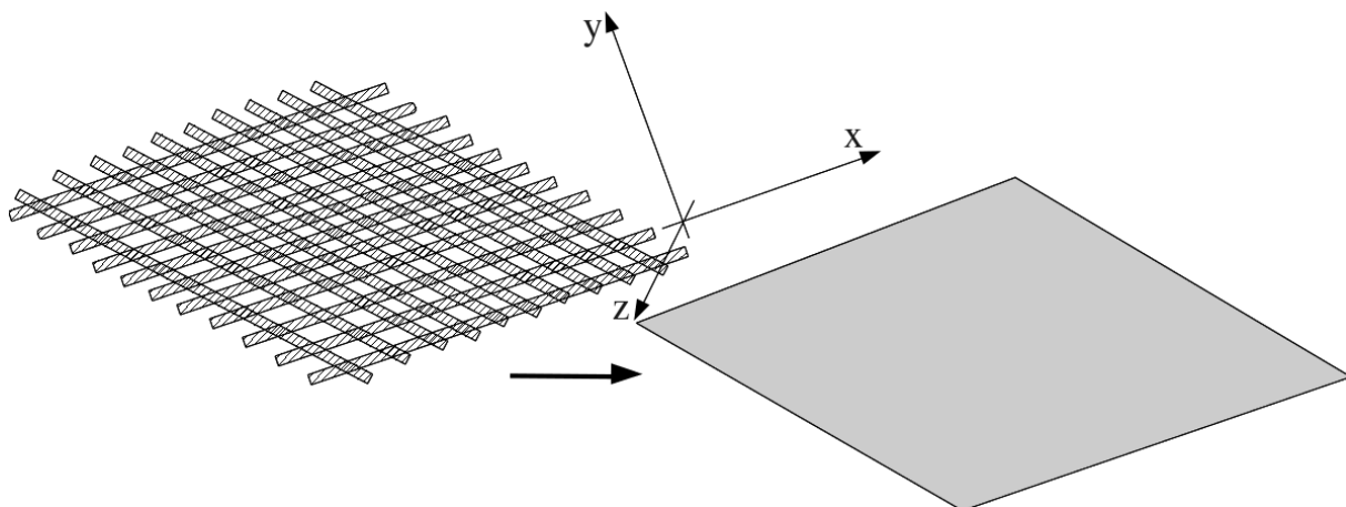
Figure 16.2-1: replacement of the reinforcements by a membrane
