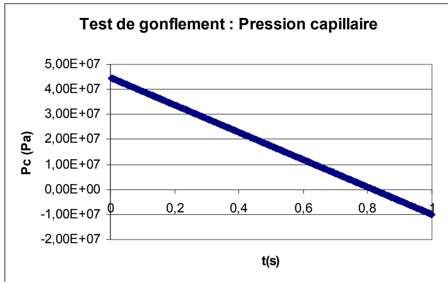
Appear 2.2-b : capillary pressure (N3)
