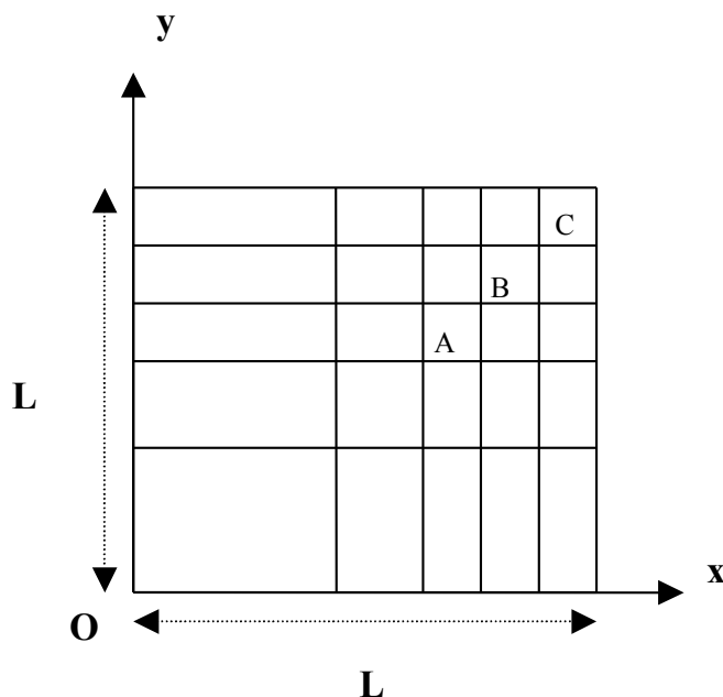
Figure 3.1-a: Geometry and mesh of the modelization
